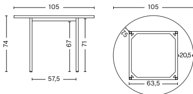
DIAMETER 105 CM | 41.34" HEIGHT 74 CM | 29.13"
