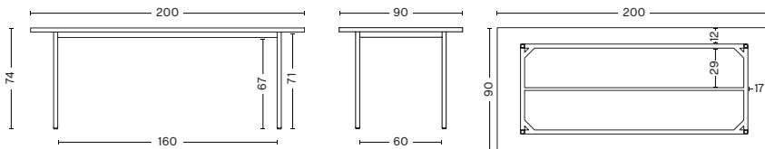
LENGTH 200 CM | 78.74" WIDTH 90 CM | 35.43" HEIGHT 74 CM | 29.13"
