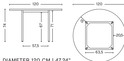
DIAMETER 120 CM | 47.24" HEIGHT 74 CM | 29.13"
