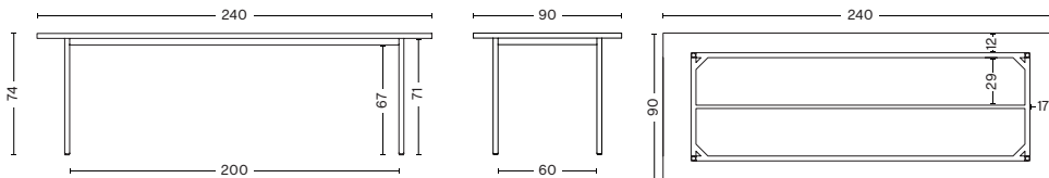
LENGTH 240 CM | 94.48" WIDTH 90 CM | 35.43" HEIGHT 74 CM | 29.13"
