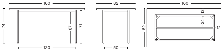
LENGTH 160 CM | 62.99" WIDTH 82 CM | 32.28" HEIGHT 74 CM | 29.13"
